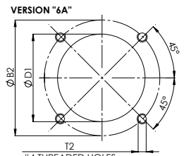
COMMON PATTERN FOR VERSIONS "6A" AND "6B"
