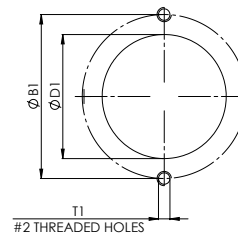
COMMON PATTERN FOR VERSIONS "6A" AND "6B"
