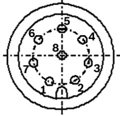
Fig. 8: Pin assignment (top view to the sensor cover)
