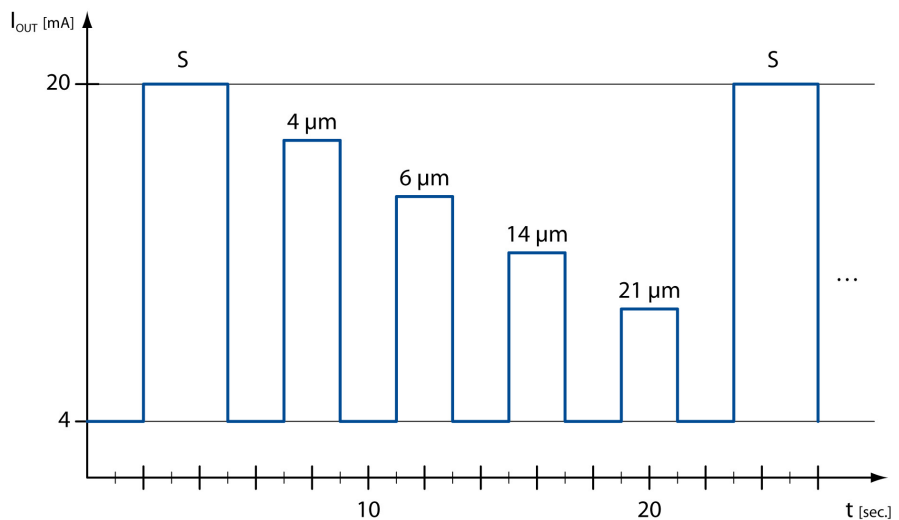
Fig. 12: Sequential data output
